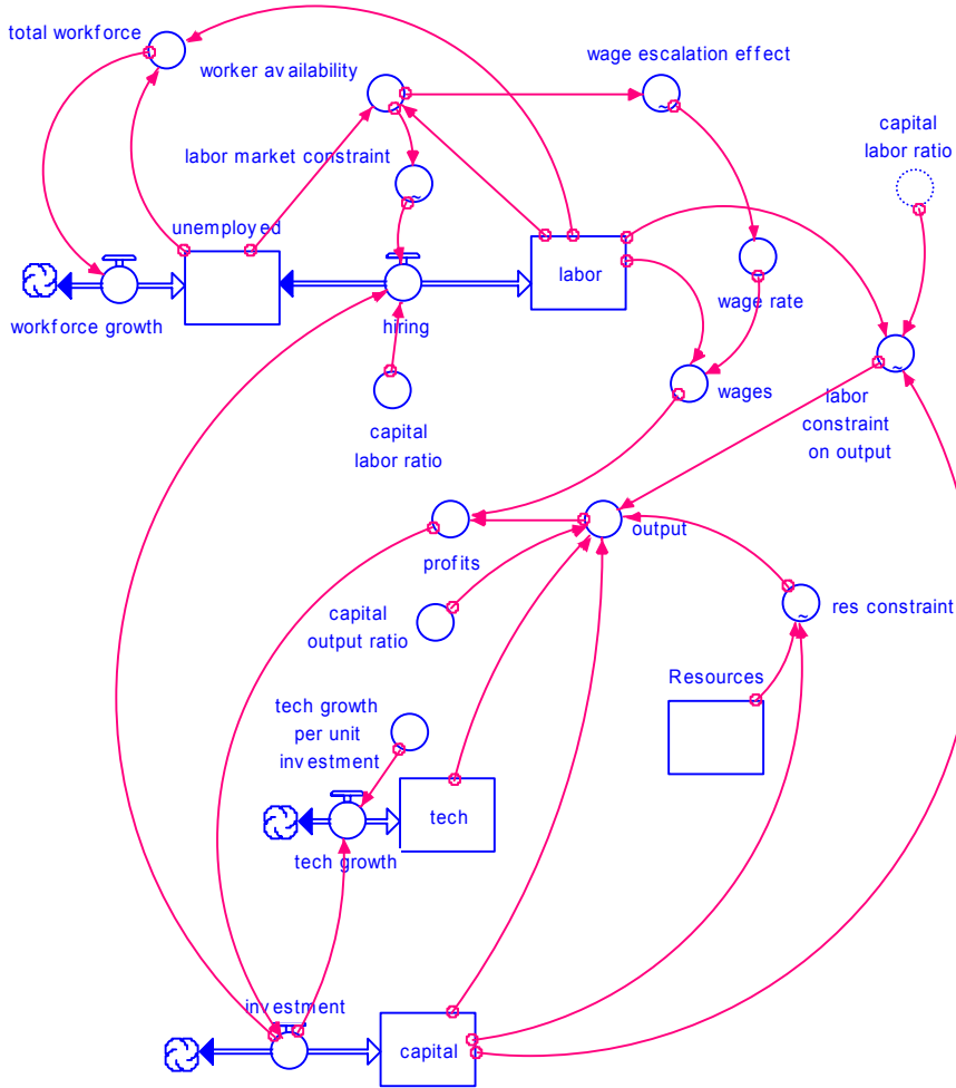
Figure 4a: Renewable resources constraint (Land) added to the model.
