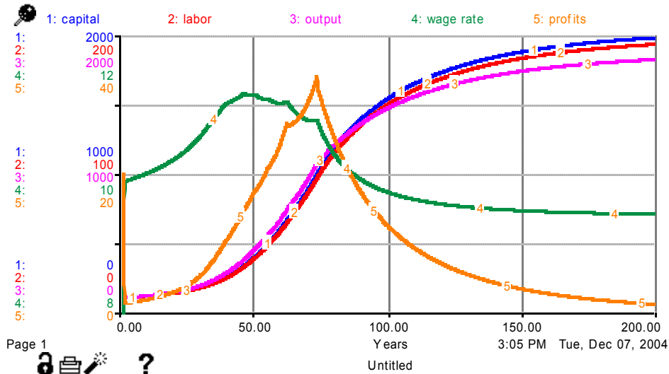
Figure 5b: Simulation of the Ricardian model of economic growth.
