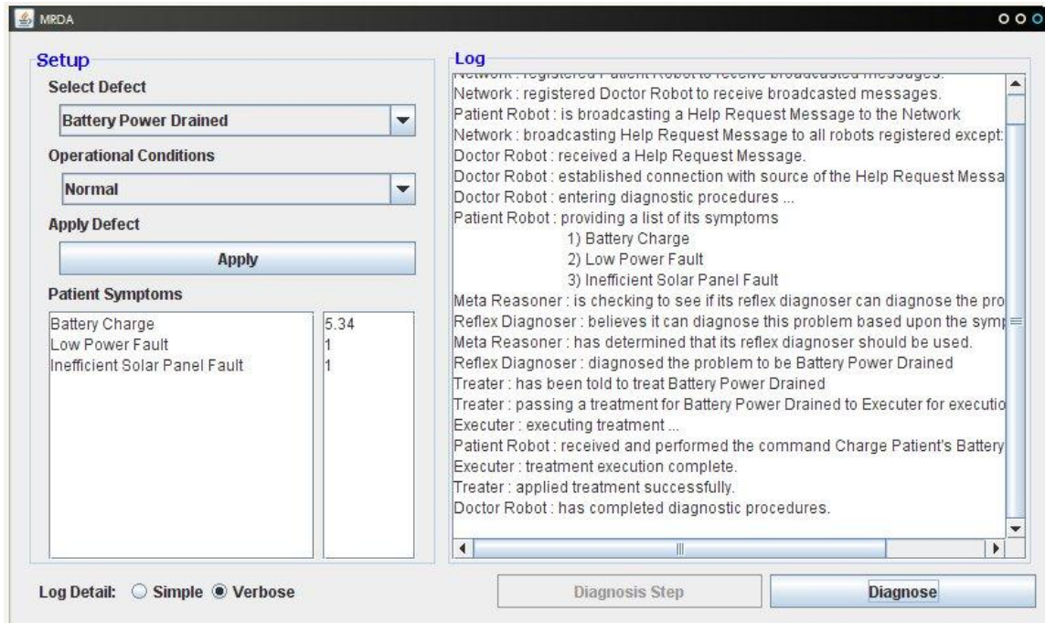
Figure 12 : Screenshot of the GUI showing an output trace
