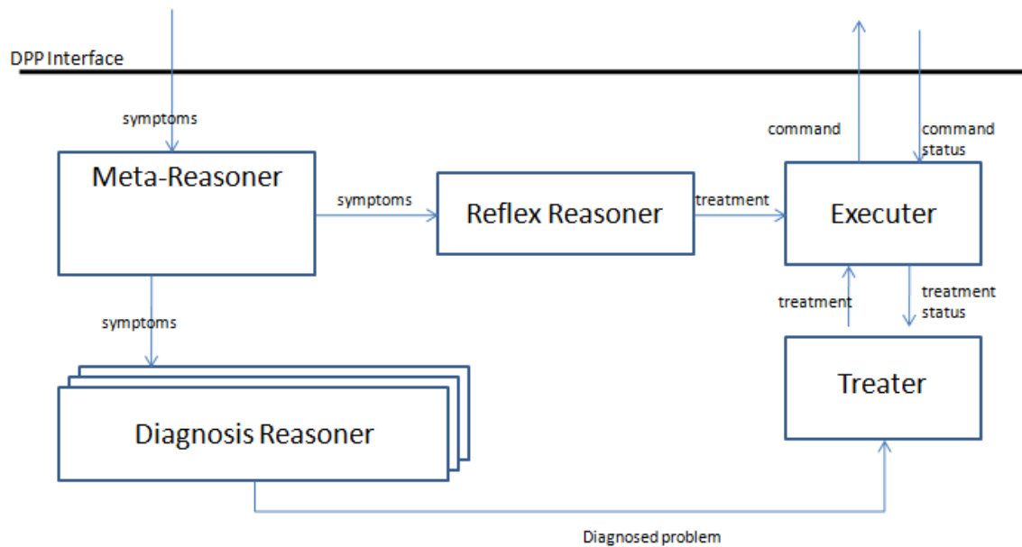
Figure 7 : Flow of data in the MRDA
