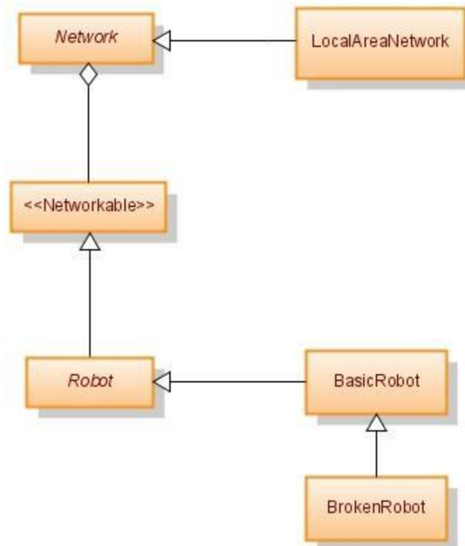
Figure 4 : High-level simulation class diagram
