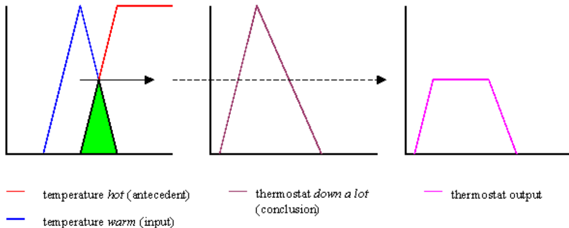
Figure 10 : Mandani Min Max Min Rule Execution (Orchard 2006)
