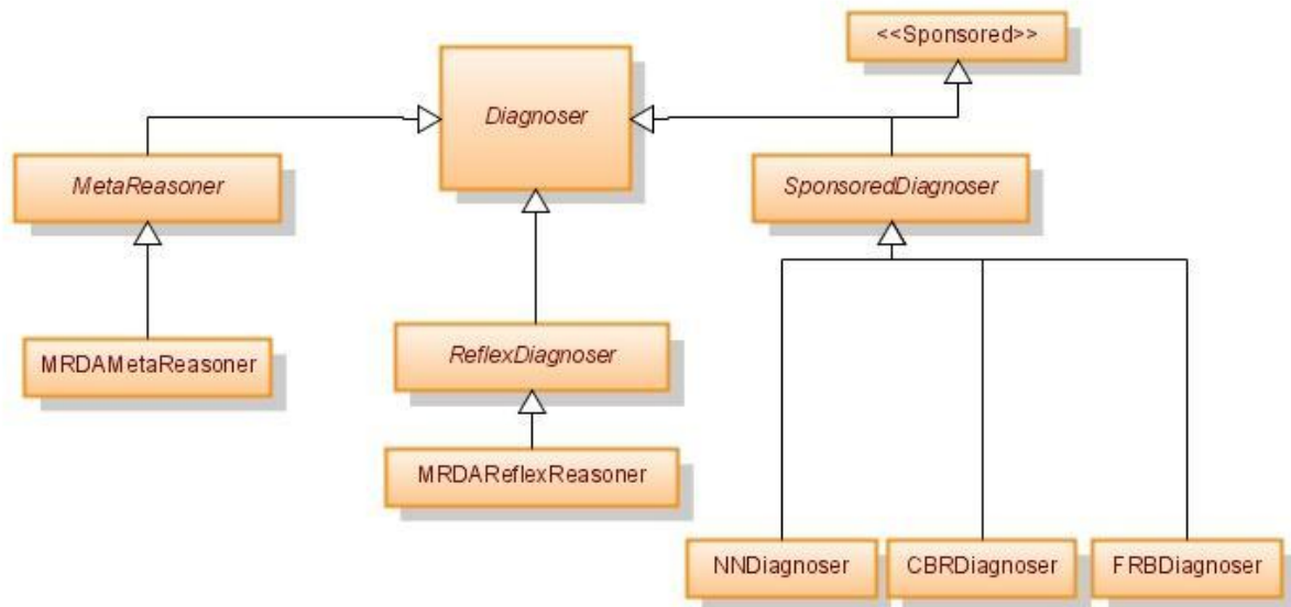
Figure 8 : Inheritance hierarchy of diagnosticians
