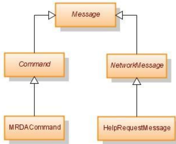
Figure 5 : Inheritance hierarchy of messages
