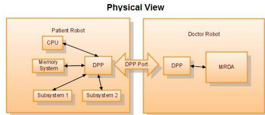
Figure 2 : High-level physical view of robot interaction via DPP
