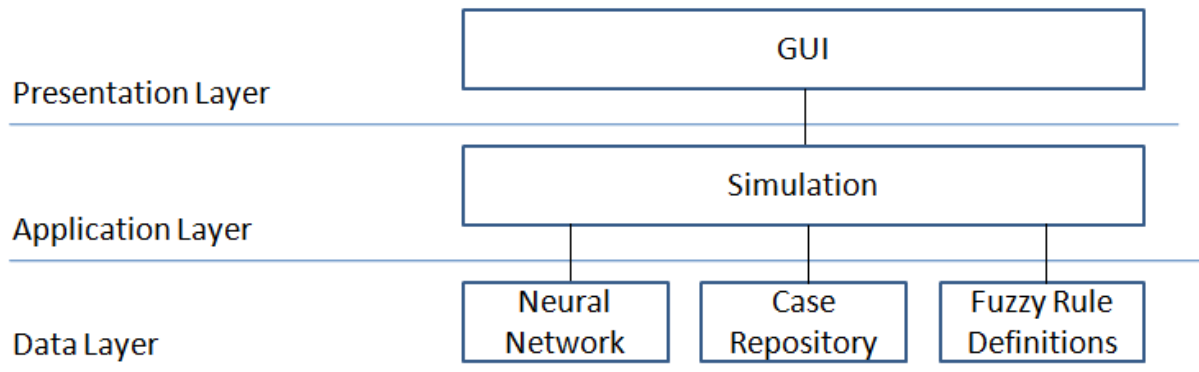
Figure 3 : High-level representation of MRDA
