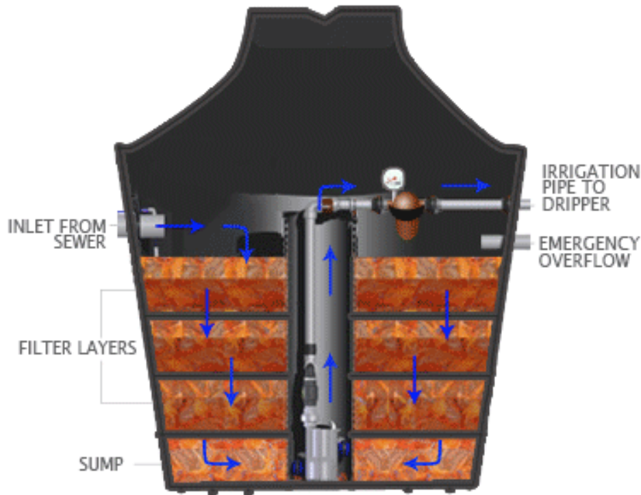
Figure 21: The Biolytix Design (Biolytix, 2009)
