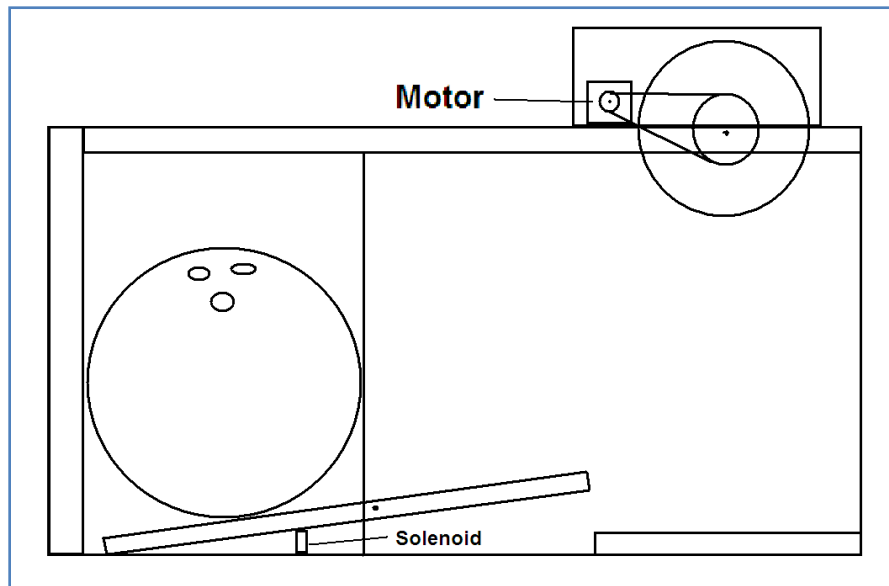
Figure 11: Side View Sketch of Ball Cannon Design
