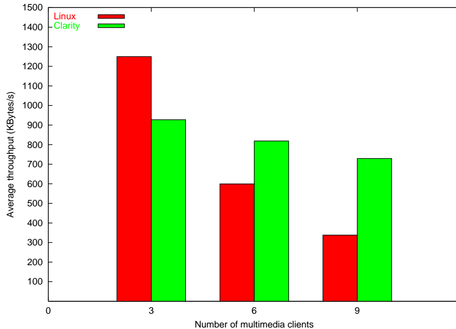
Figure 5.17: Average throughput for non-multimedia clients under Linux and Clarity in the presence of excess multimedia clients
