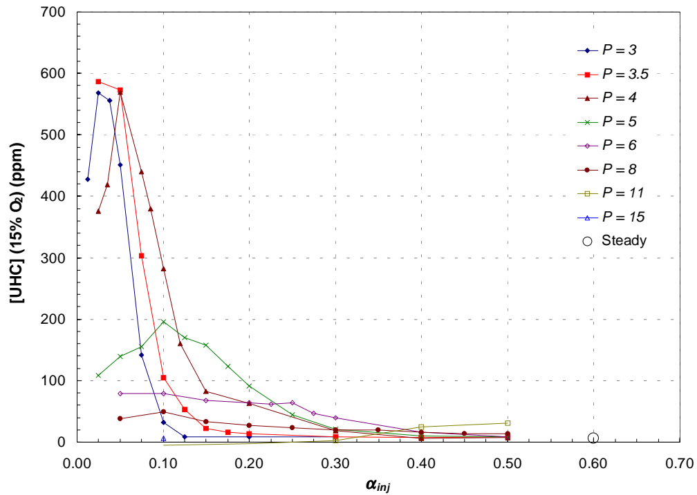
Figure 6.7: Corrected average UHC concentrations
