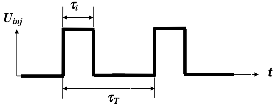
Figure 2.4: Ideal pulse cycle
