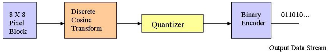
Figure 2.1: JPEG Compression
