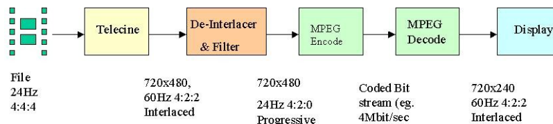
Figure 2.2: MPEG Compression
