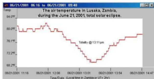
Air-temperature plummets significantly during a solar eclipse. Picture credit: NASA
