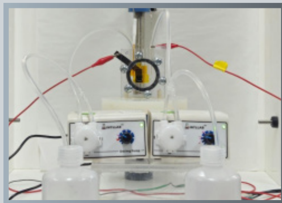
The prototype fluidic cell developed by Prof. Teng's research group is used for the electrochemical recovery of critical materials
