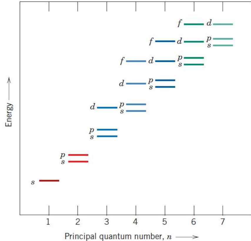
wave-mechanical model
