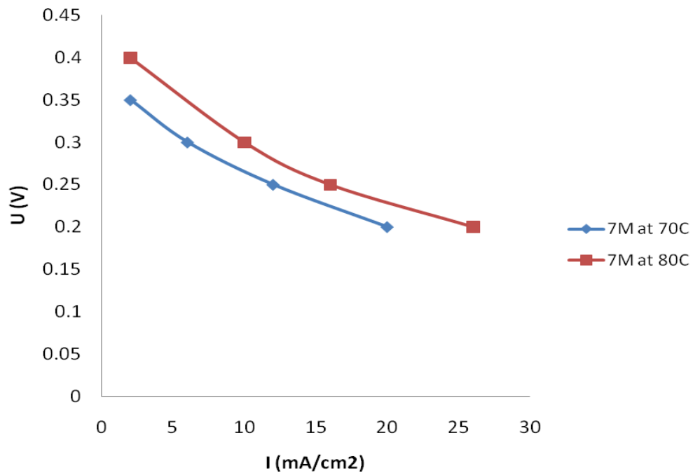
Figure 32. Results of testing a Nafion 1035 membrane with 7M feed at different temperatures.
