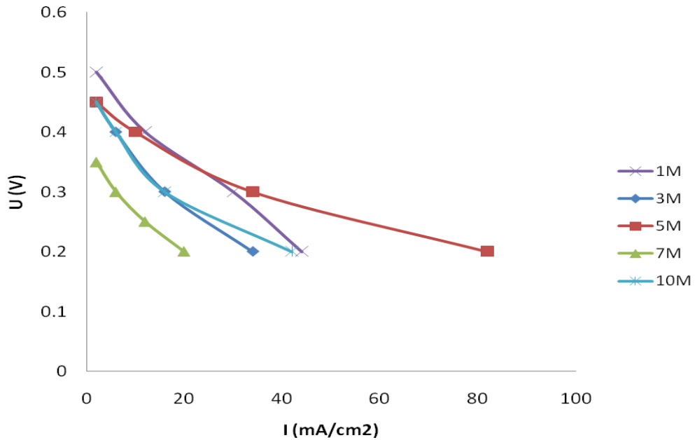
Figure 27. Results of testing a Nafion 1035 membrane with ElectroChem electrodes at different methanol feed concentrations and at 70 °C.
