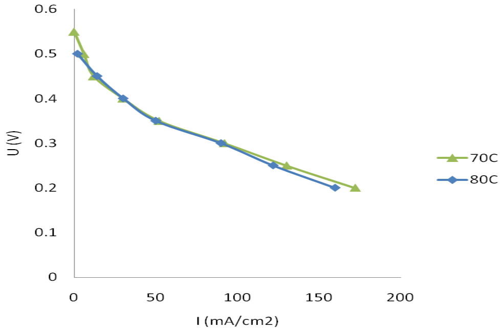
Figure 29. Results of testing a Nafion 115 membrane with 7M feed at different temperatures.
