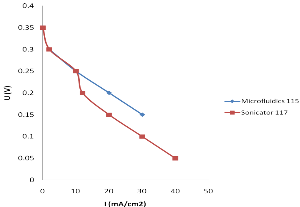
Figure 23. Comparison at 70 °C between a Nafion 117 membrane with catalyst ink prepared in a sonicator with a Nafion 115 membrane with ink prepared in the Microfluidizer.
