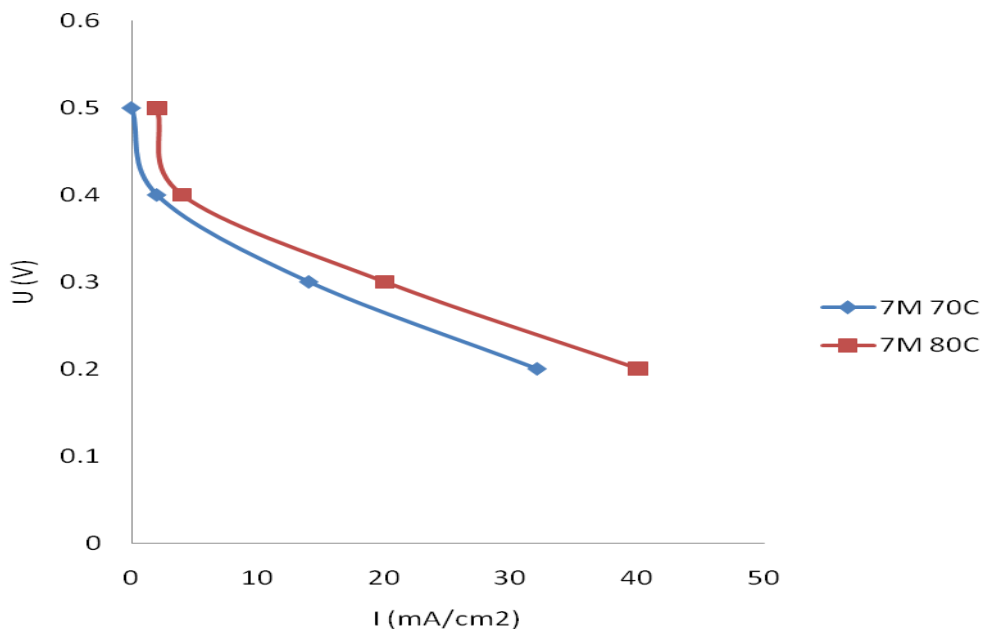
Figure 30. Results of testing a Nafion 117 membrane with 7M feed at different temperatures.
