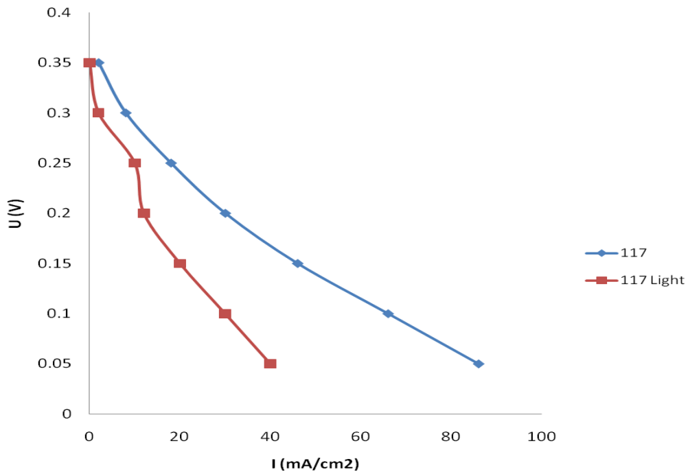
Figure 21. Difference in performance between opaque and less opaque catalyst ink application on a Nafion 117 membrane at 70°C.
