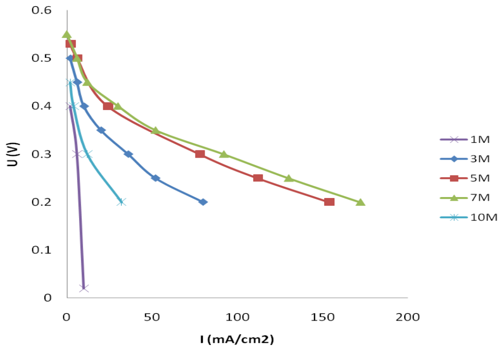
Figure 24. Results of testing a Nafion 115 membrane with ElectroChem electrodes at different methanol feed concentrations and 70 °C.
