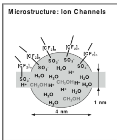
Figure 4. Ion channel (water-filled micropore) in Nafion (Schultz, 2001).
