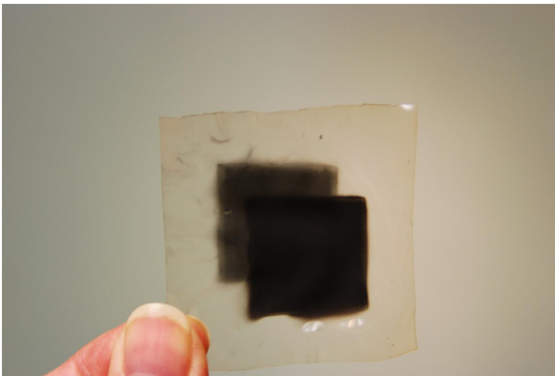
Figure 20. Nafion membrane with anode and cathode ink applied. The anode ink is lighter than the cathode ink application.
