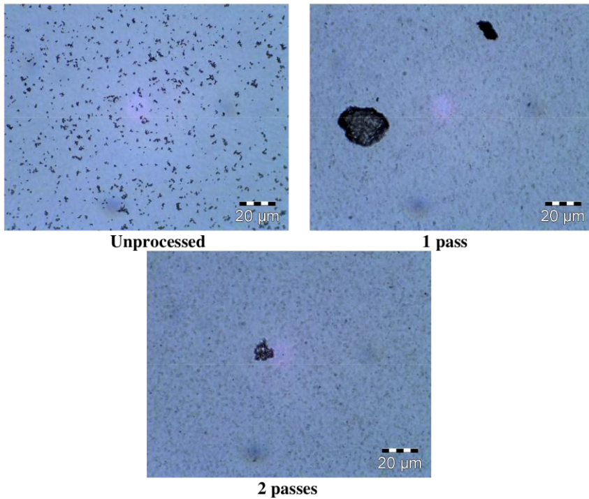
Figure 22. Images of cathode catalyst ink after various stages of processing in the M-110S Microfluidizer at 20,000 psi with the F12Y interaction chamber.
