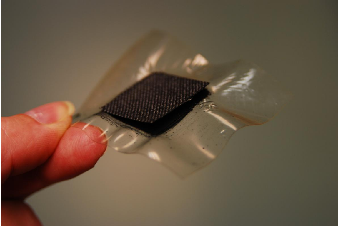
Figure 13. A used Nafion membrane with slightly detached ElectroChem electrodes pressed on either side of the membrane.
