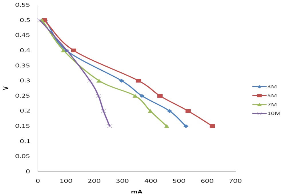
Figure 19. Performance of a commercial E-Tek MEA at four different methanol molar concentrations and a cell temperature of 70 °C.
