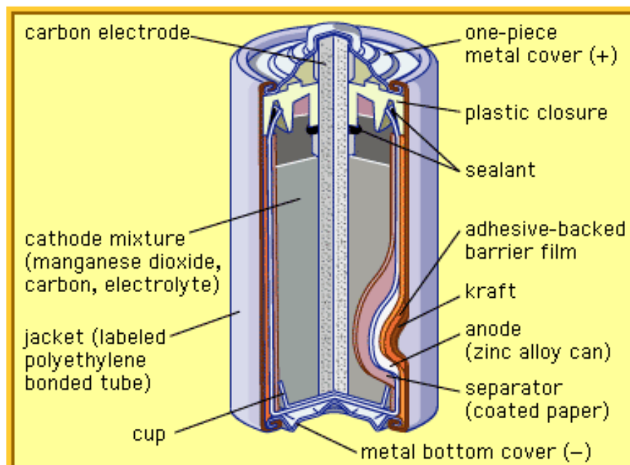
Figure 1. Schematic of a Zinc-Carbon battery. (Encyclopedia Britannica, Inc., 2005).
