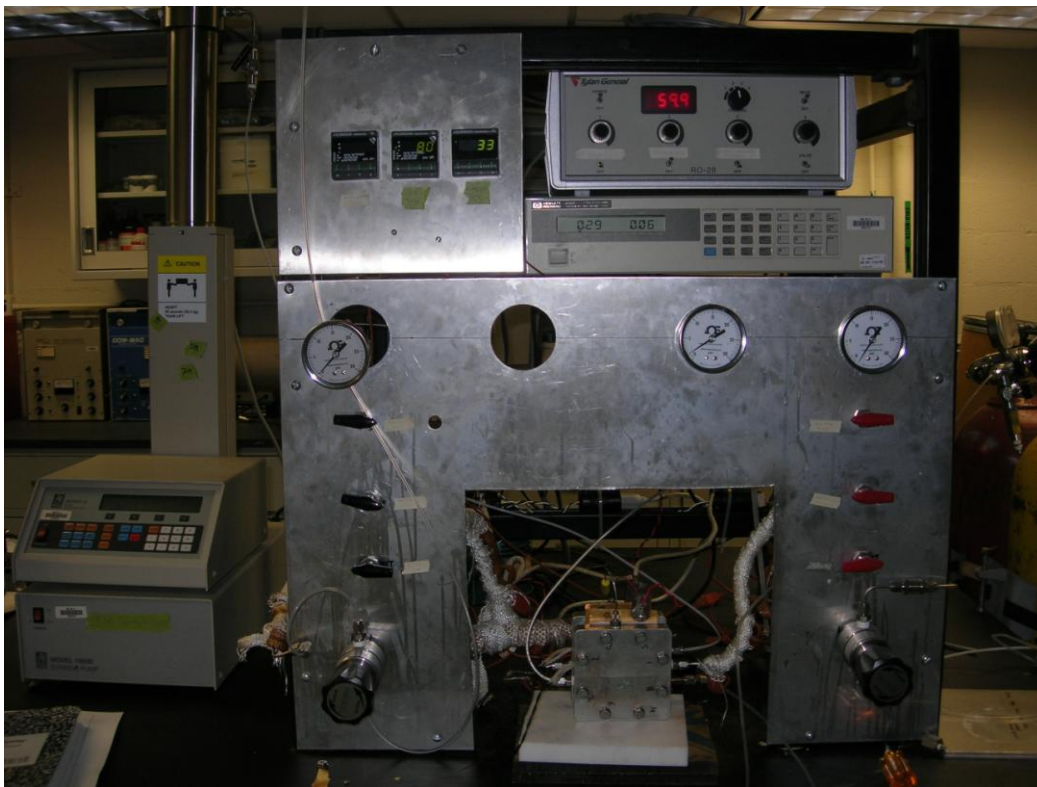
Figure 17. The fuel cell testing station with methanol fuel pump on the left.
