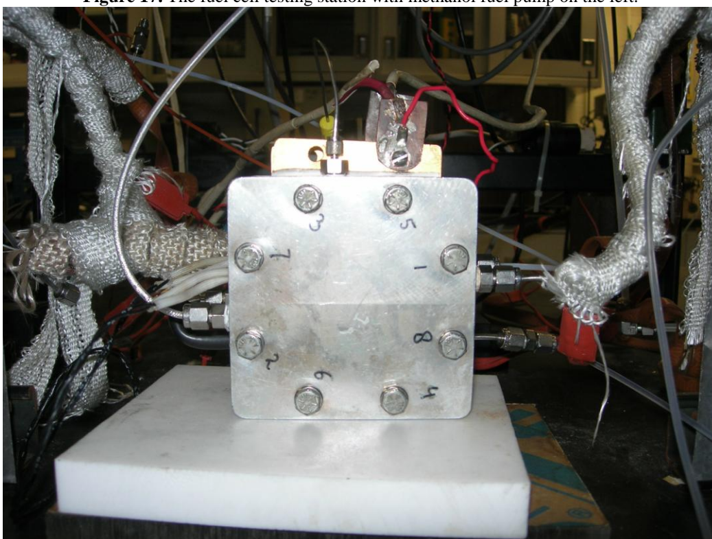
Figure 18. The fuel cell assembly hooked up to the testing station.
