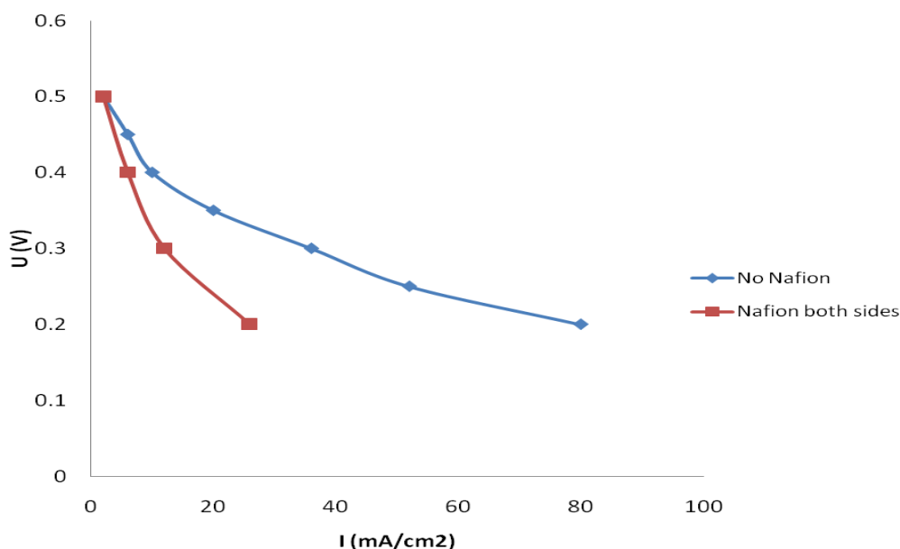
Figure 34. Comparison between 115 membranes with commercial electrodes with and without added 10 wt% Nafion solution.
