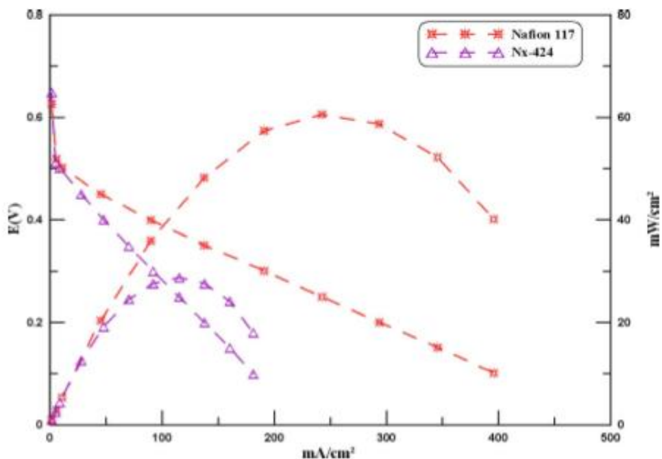
Figure 6. Performance of Nafion 117 compared to Nx-424 at 2 M methanol 5 cc/min and 70 °C, oxygen at 150 cc/min (Jung et al., 2007).
