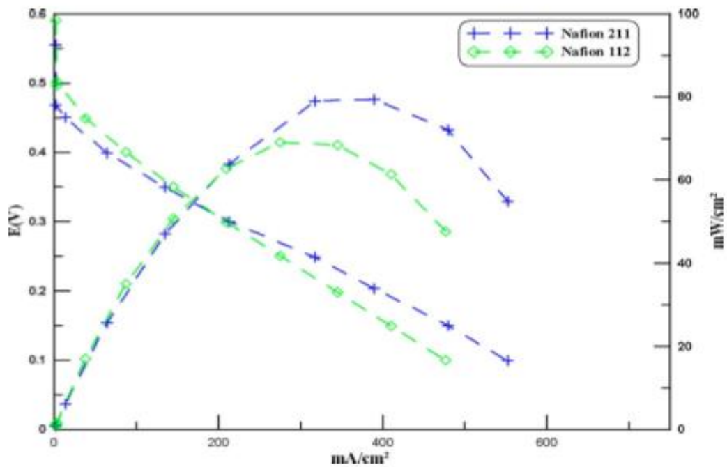
Figure 5. Performance of Nafion 211 compared to Nafion 112 at 2M methanol 5 cc/min and 70°C, oxygen at 150 cc/min (Jung et al., 2007).
