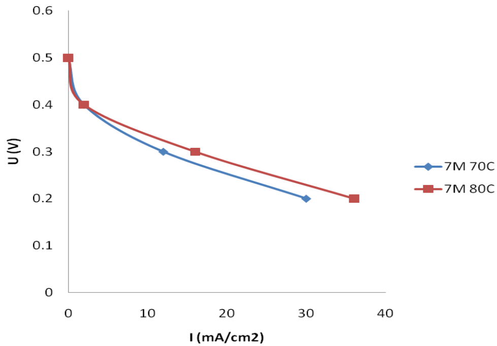
Figure 31. Results of testing a Nafion 1110 membrane with 7M feed at different temperatures.
