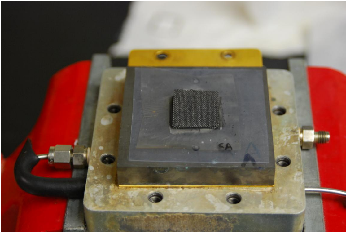
Figure 15. Anode bipolar plate with Teflon gasket and MEA aligned.
