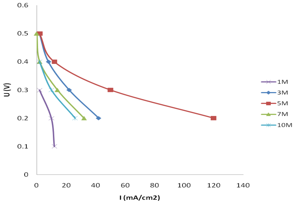
Figure 25. Results of testing a Nafion 117 membrane with ElectroChem electrodes at different methanol feed concentrations and at 70 °C.
