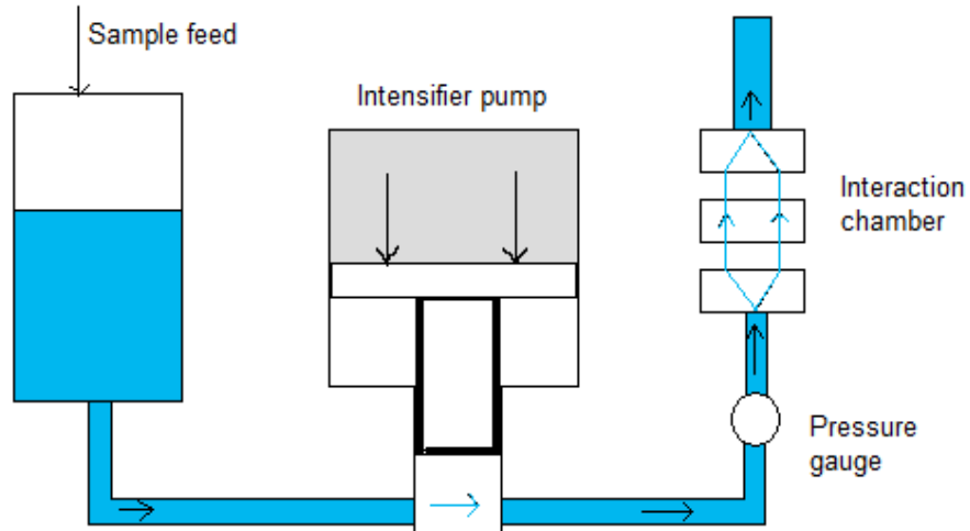
Figure 11. Schematic of a standard Microfluidizer Processor.
