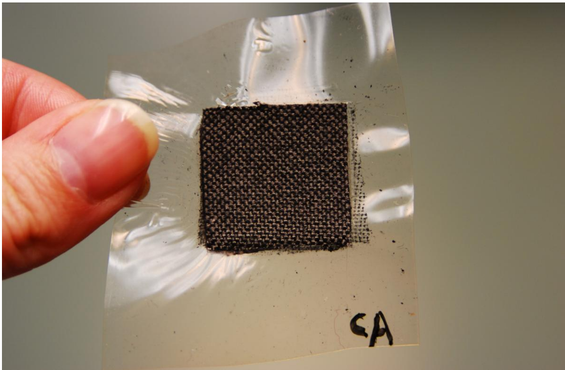
Figure 7. Front view of the cathode side of a MEA with a Nafion membrane and a carbon cloth electrode.
