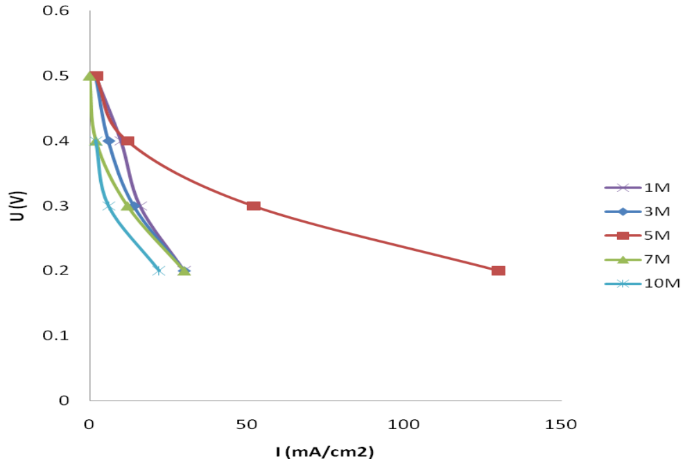
Figure 26. Results of testing a Nafion 1110 membrane with ElectroChem electrodes at different methanol feed concentrations and at 70 °C.
