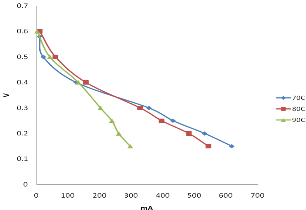
Figure 28. Results of commercial E-Tek MEA at different temperatures with a 5M methanol feed.
