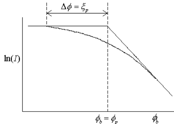
Figure 4.4: Characteristic I-V curve of a voltage sweep measurement of the plasma potential (occurring at the “knee” in the plot), illustrating the potential drop across the sheath.
