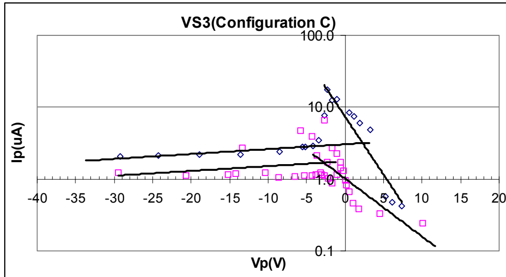
Figure 3.12: Case VS3 V-I characteristic. The pink squares represent the spray turned off, and the blue diamonds represent the spray turned on (probe is 2.7cm from electro spray). Probe current uncertainty is within \pm 20\text{nA} , probe potential uncertainty is within \pm 0.24\text{V} .
