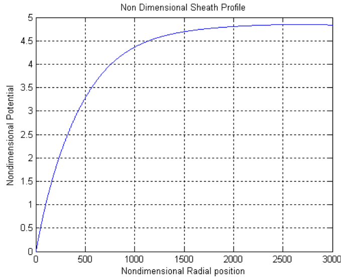
Figure 4.2: Typical results showing the solution to \xi . Note \theta (theta) begins at the nonzero point equivalent to r = r_o . For the case shown, \xi_p = 5 , n_o = 10^5 \text{ cm}^{-3} , r_o = 0.00381 \text{ cm} , T_w = T_e = 2500 \text{ K} and i/l = 7.95 \mu\text{A/cm} .
