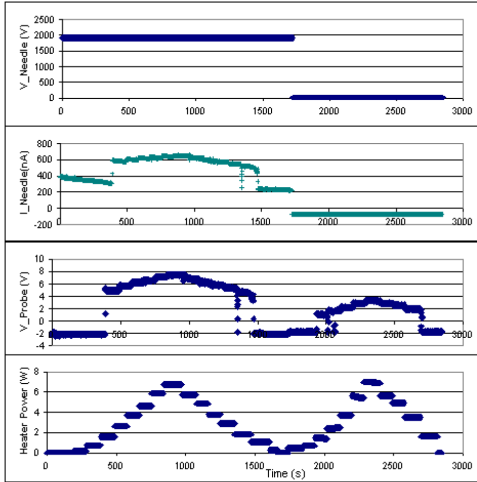
Figure 3.9: Telemetry channels from Case FP3 floating probe test. Heater power uncertainty is \pm 0.75\text{W} , floating potential is at \pm 0.24\text{V} and electro spray and extractor currents are accurate to \pm 3.61\text{nA} and \pm 0.43\text{nA} , respectively.
