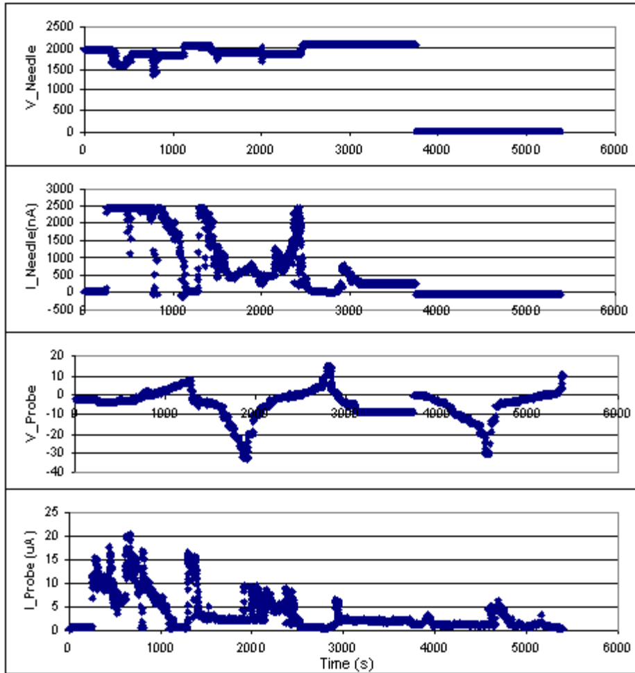
Figure 3.13: Telemetry from case VS3 (configuration C). Needle voltage uncertainty is \pm 9.63\text{V} , needle current uncertainty is \pm 3.61\text{nA} , probe potential uncertainty is within \pm 0.24\text{V} and probe current uncertainty is within \pm 20\text{nA} .
