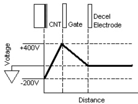
Figure 2.7: Potential energy diagram of cathode emitter similar to electrospray diagram.
