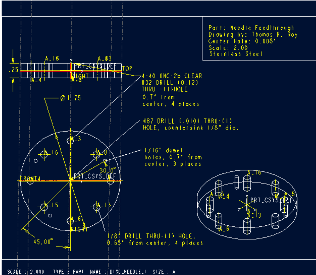
Figure A.2: This needle housing was originally going to be stainless steel for the purpose of conducting current to the needle tip, however it was later determined that Delrin plastic would isolate the needle while providing mechanical support: the current was applied externally to the needle. This representation is not to the reported scale.
