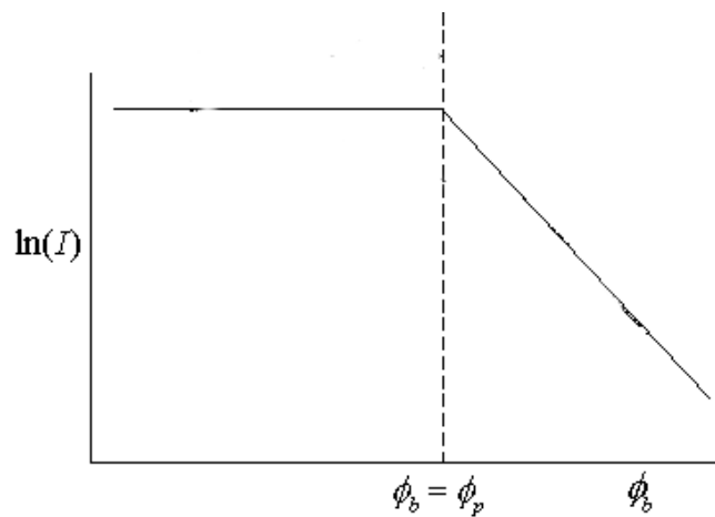
Figure 1.3: Sketch of a voltage sweep technique characteristic curve of the current drawn by the emissive probe plotted against the probe bias potential.
